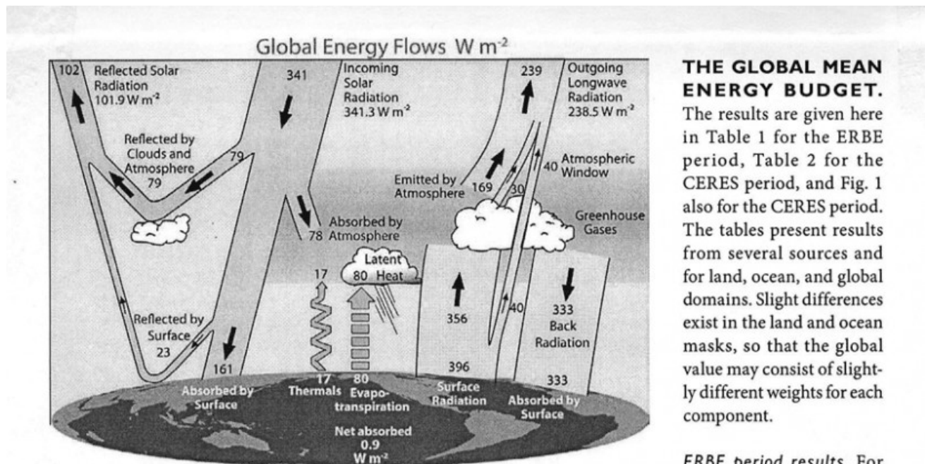
FIG. 1. The global annual mean Earth's energy budget for the Mar 2000 to May 2004 period ( W m^{-2} ). The broad arrows indicate the schematic flow of energy in proportion to their importance.
