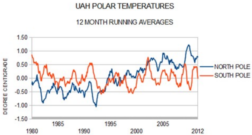
FIG.2. 12 month running averages temperatures for The North Pole and South Pole by The University of Alabama in Huntsville Polar Temperatures 1980-2012
