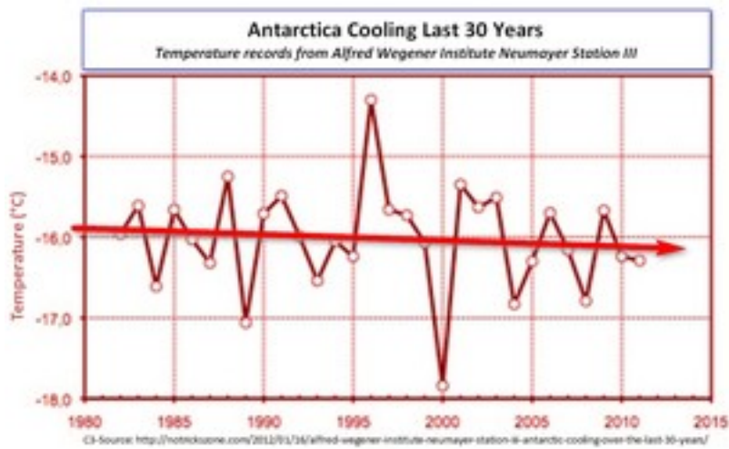
Fig.3. Temperature records from antarctic station III of Alfred Wegener Institute in Neumayer for the last 30 years
